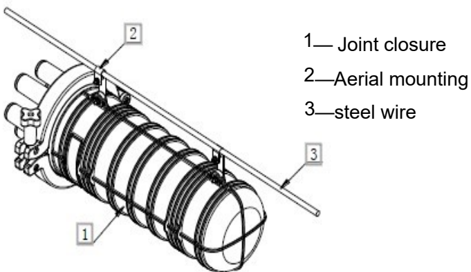
Aerial mounting
